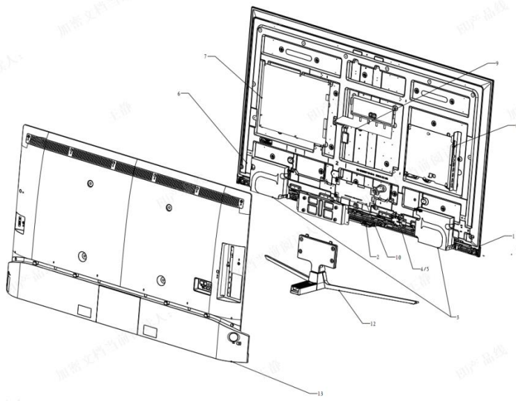
The explosive view of 55/65 explosive view
